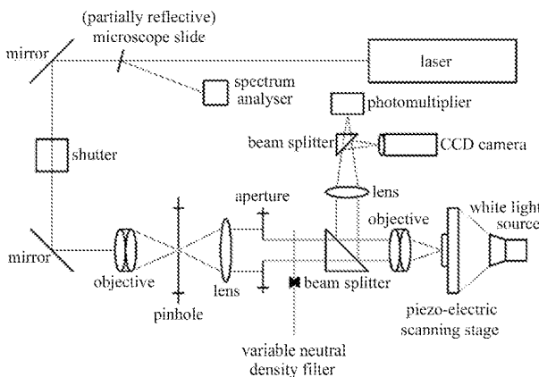
Fig. 1. Experimental set up for micro-fabrication.
