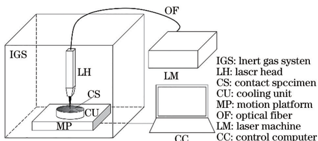
图 2 激光表面快速熔凝改性实验系统示意图 Fig. 2 Schematic diagram of laser surface remelting experimental system
