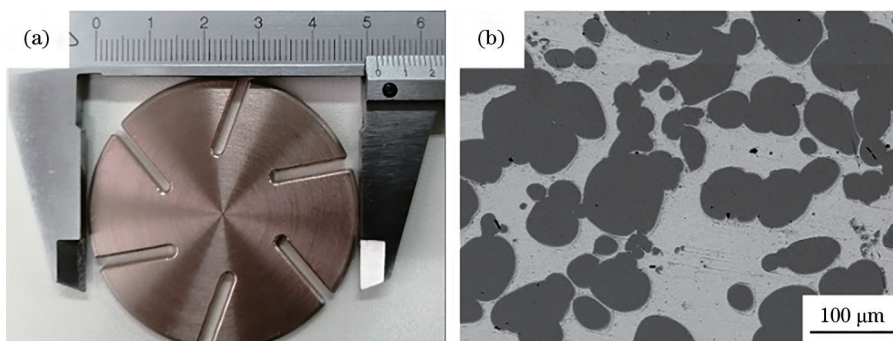
图 1 CuCr50 合金。(a)触头原件;(b)微观组织 Fig. 1 CuCr50 alloy. (a) Contact specimen; (b) microstructure
