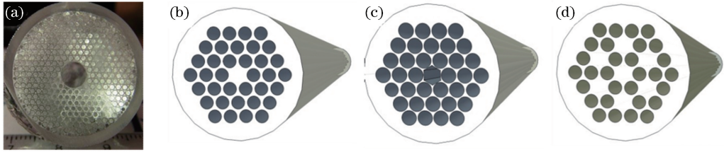
图3 毛细管堆叠技术。(a)空芯微结构光纤预制棒端面的照片;(b)实芯光纤;(c)空芯带隙光纤;(d)多芯光纤 Fig. 3 Capillary stacking technology. (a) Cross section of hollow core microstructure optical fiber preform; (b) solid core fiber; (c) hollow core bandgap fiber; (d) multicore fiber
