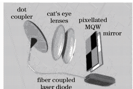
图 7 具有发射器/接收器的 CE MRR Fig. 7 Diagram of CE MRR with transmitter/receiver
