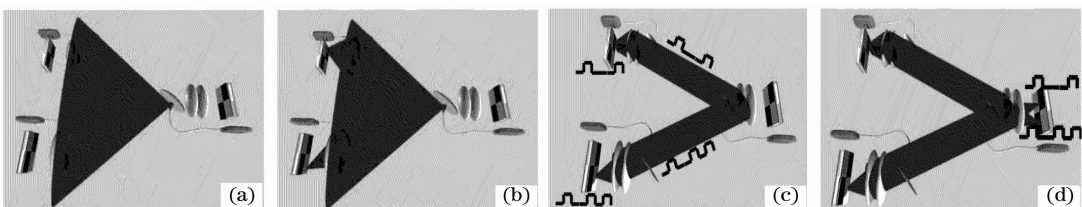
图 8 具有发射器/接收器的 CE MRR 构成通信链路过程 Fig. 8 Communication link process of CE MRR with transmitter/receiver
