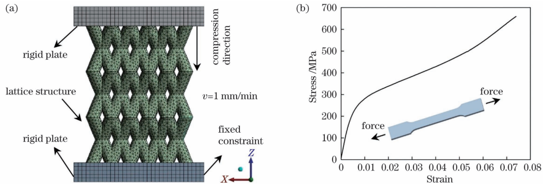
图 3 有限元模拟及单轴拉伸曲线。(a) 网格划分和边界条件; (b) NiTi 合金单轴拉伸应力-应变曲线, 插图 LPBF 制成的拉伸件 Fig. 3 Finite element simulation and uniaxial tensile curve. (a) Meshing and boundary conditions; (b) uniaxial tensile stress-strain curve with LPBF processed tensile sample shown in inset
