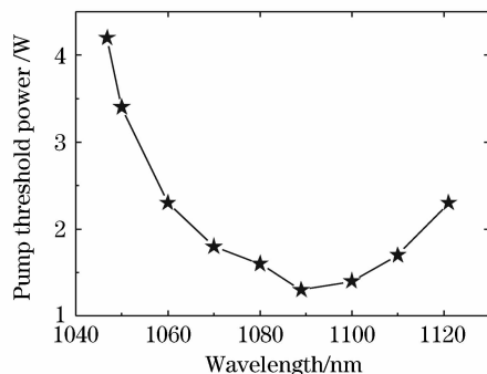
图4 不同调谐波长处的入纤抽运阈值功率 Fig. 4 Threshold pump power with different lasing wavelengths
