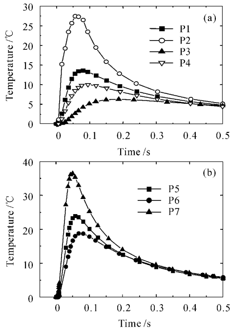
图 6 对应不同输入点的计算温度响应曲线 Fig. 6 Calculated temperature changes with time for different points
