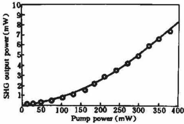
Fig. 2 SHG output versus pump power
