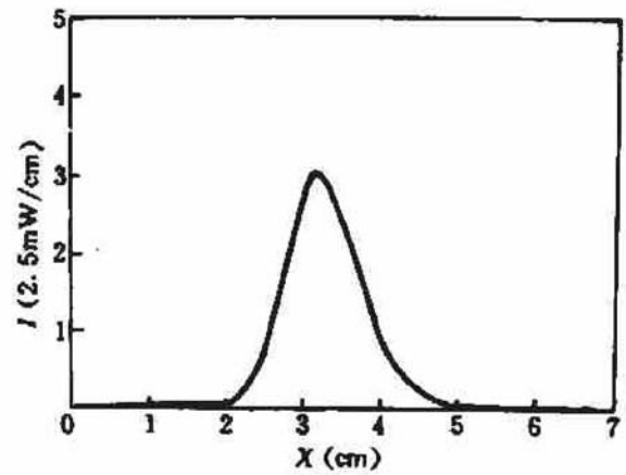
Fig. 3 Intensity profile of SHG output
