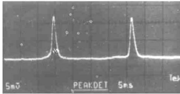
Fig. 4 Optical spectrum of single-frequency operation at 532 nm measured by using a scanning confocal interferometer with 735 MHz free spectral range
