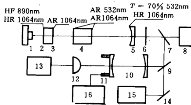
Fig. 1 Experimental setup
