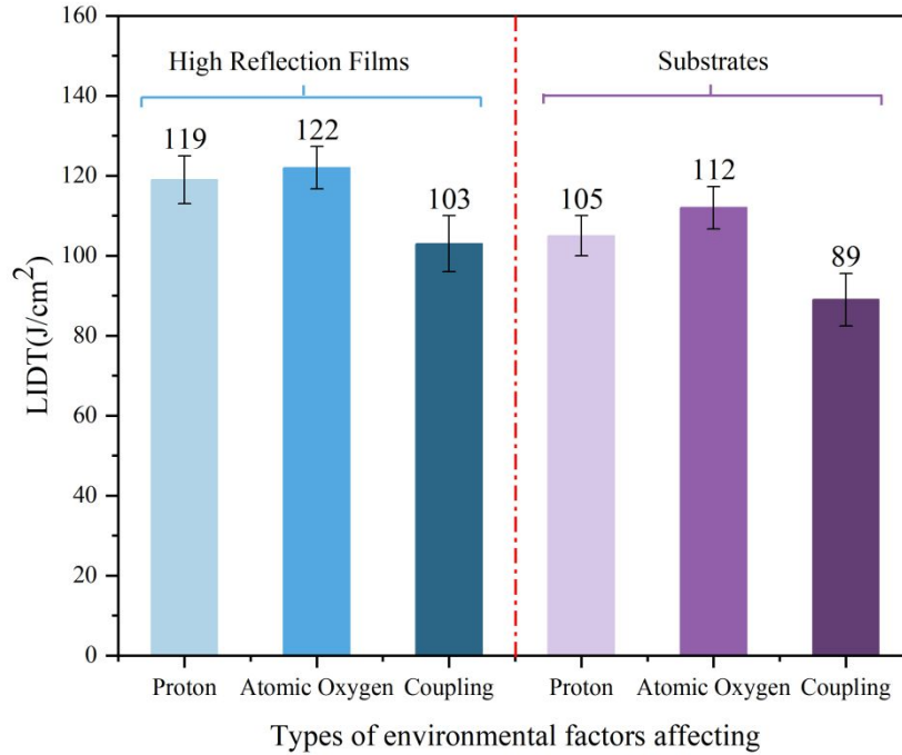
Fig. 6. A comparison of LIDT values produced by the coupled effect of atomic oxygen and protons.
